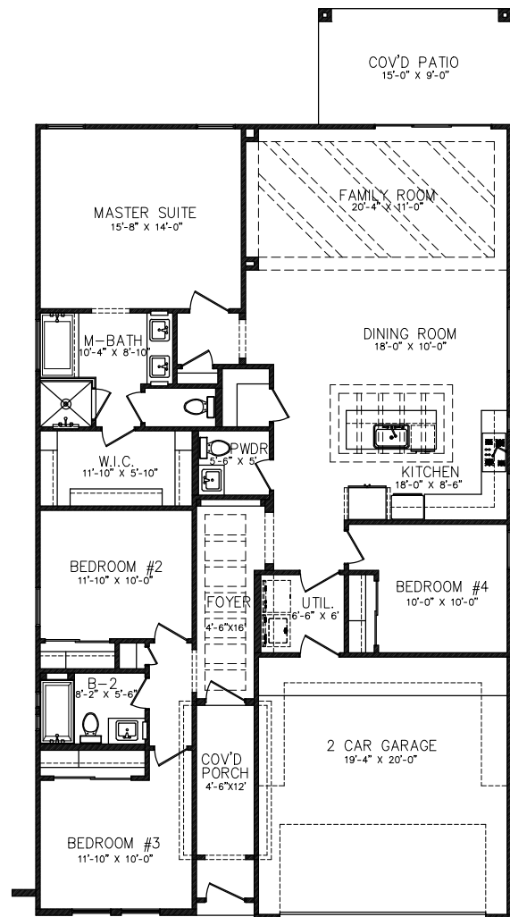
FLOOR PLAN
