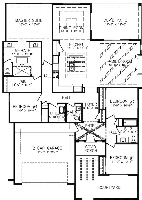
FLOOR PLAN
