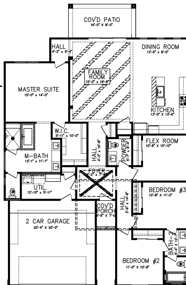
FLOOR PLAN
