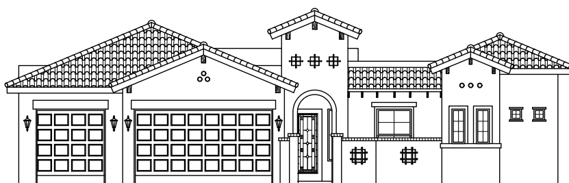
FRONT ELEVATION
