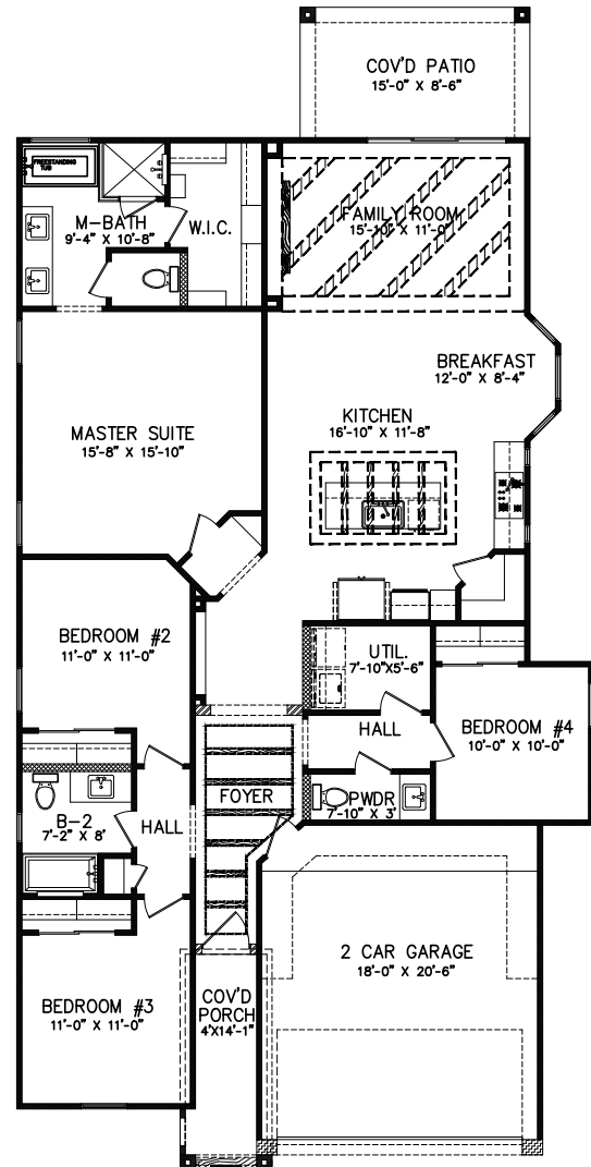
FLOOR PLAN
