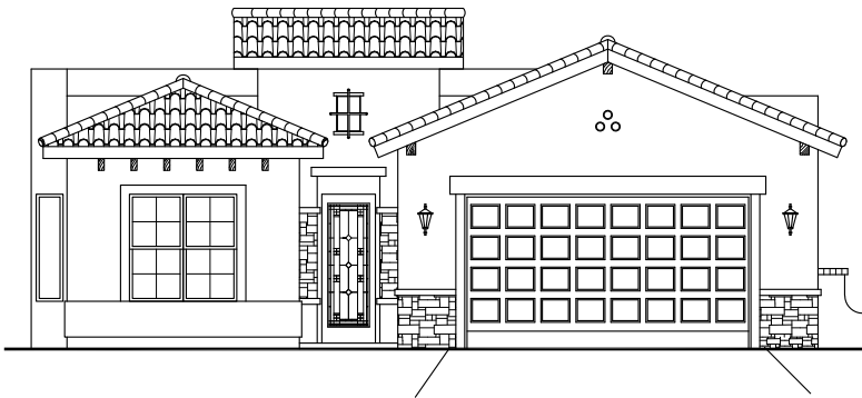
FRONT ELEVATION
