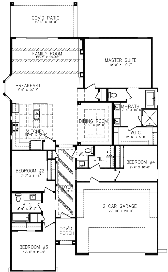
FLOOR PLAN
