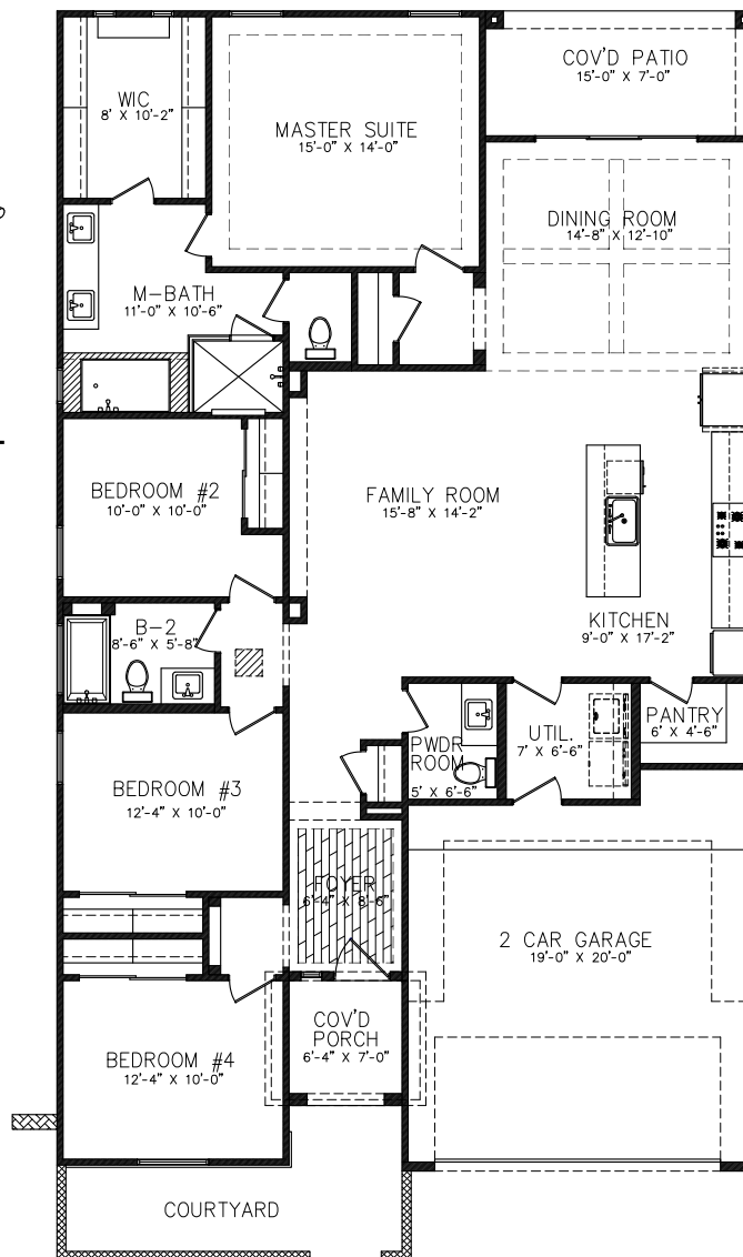
FLOOR PLAN
